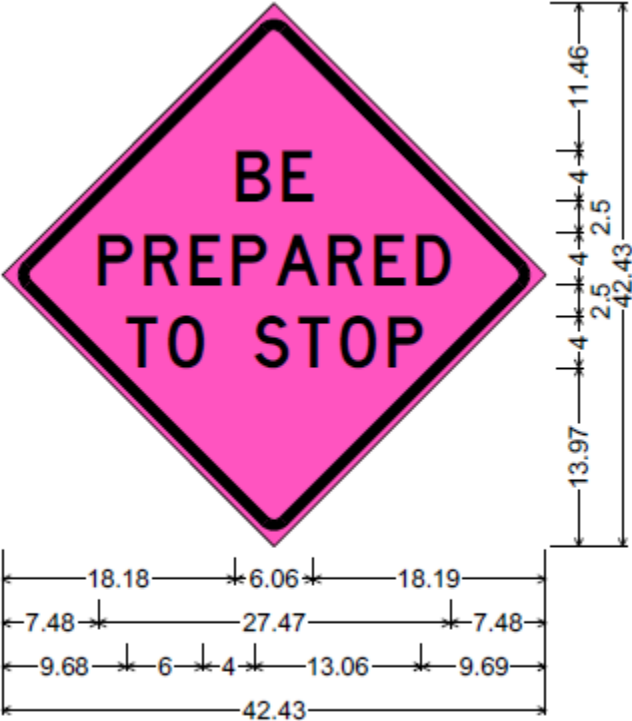
Identifier : W3-4_30x30 30.00" across sides 0.75" Border, 0.50" Indent, Black on Pink; "BE" D; "PREPARED" D; "TO STOP" D;
